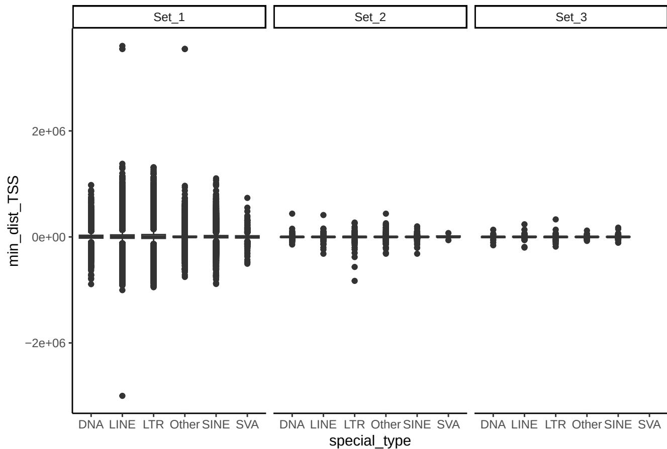
Distance to TSS per class in H3K9me3 of overlapping ROIs
